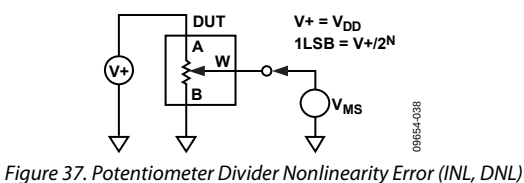
Figure 37. Potentiometer Divider Nonlinearity Error (INL, DNL)
