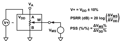
Figure 39. Power Supply Sensitivity (PSS, PSRR)
