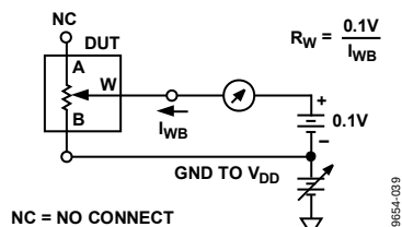
Figure 38. Wiper Resistance
