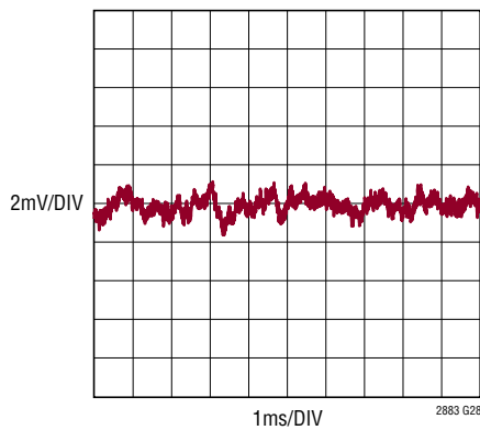
V_{CC2} Noise
