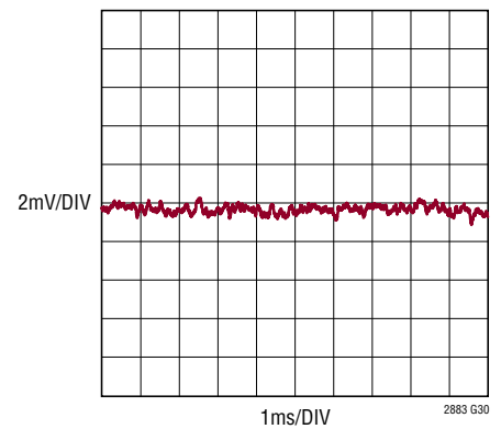
V^- Noise
