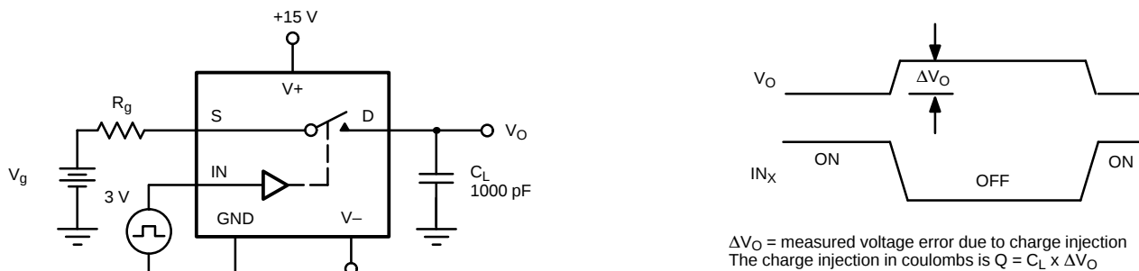
FIGURE 3. Charge Injection
