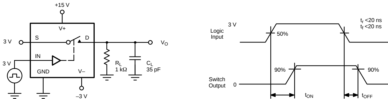
FIGURE 2. Switching Time
