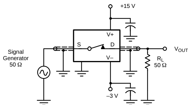
FIGURE 6. Bandwidth
