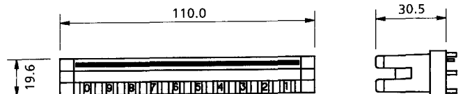
10 Pair PCB Disconnection Module
