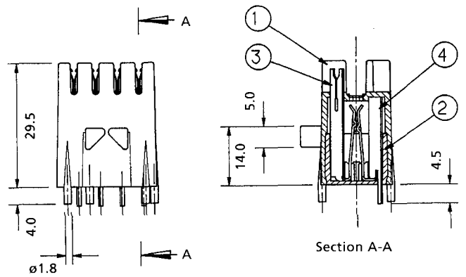
2 Pair Disconnection Module
