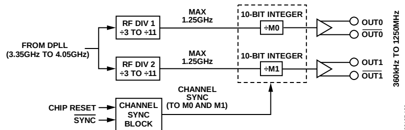
Figure 40. Clock Distribution Block Diagram
