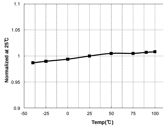
Figure 13. \text{V}_{\text{CSSH}} vs. Temperature
