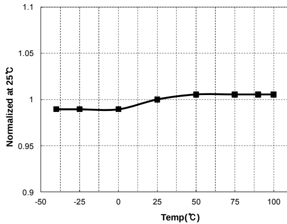
Figure 12. \text{V}_{\text{CSSL}} vs. Temperature
