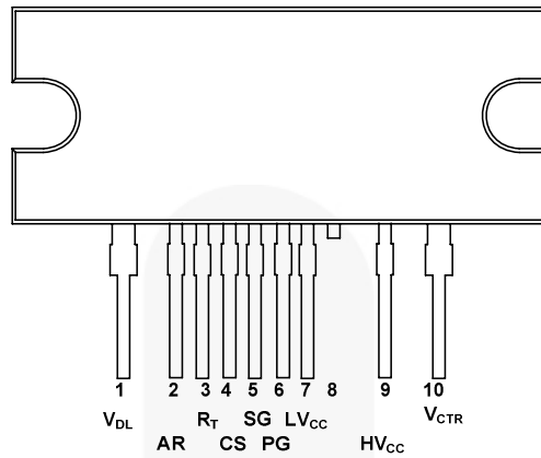
Figure 3. Package Diagram
