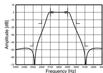
CF-4FPA 2800Hz
