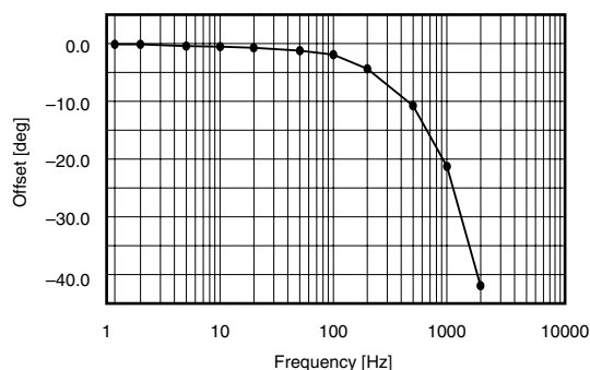
Phase offset
