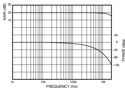
Amplitude-Phase ( \times 10 gain)
