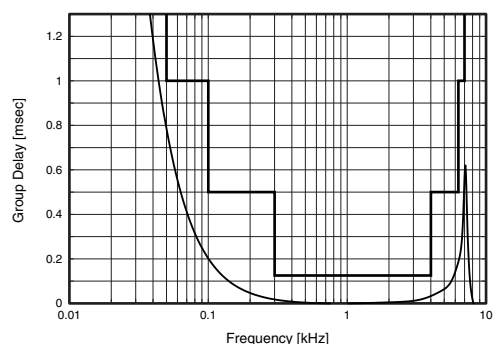
Measured group delay response
