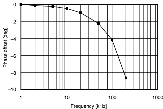
Phase offset
