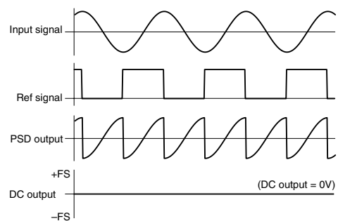
I/O waveform (Phase difference: 270^\circ )
