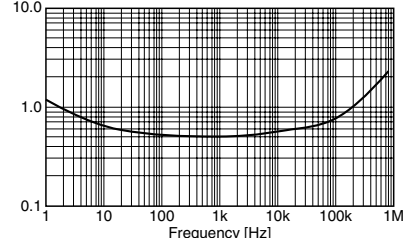
SA-400F3: Input voltage noise density
