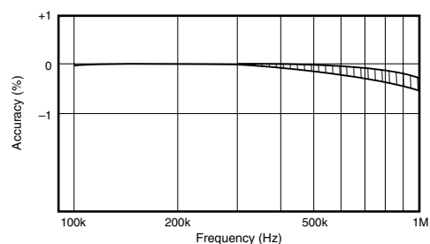
Oscillation frequency accuracy 100kHz standard: R F : Calculated value
