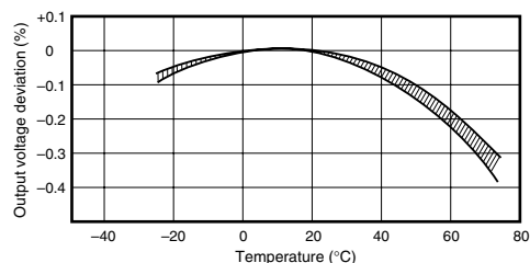
Output voltage - Temperature f_o = 1\text{MHz}
