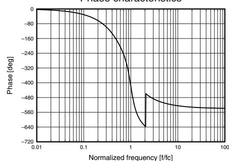
Phase characteristics
