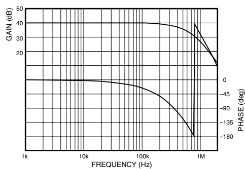
Amplitude-Phase ( \times 100 gain)
