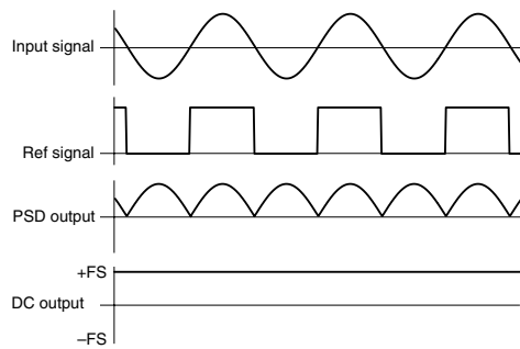
I/O waveform (Phase difference: 0^\circ )
