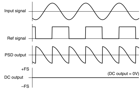
I/O waveform (Phase difference: 90^\circ )
