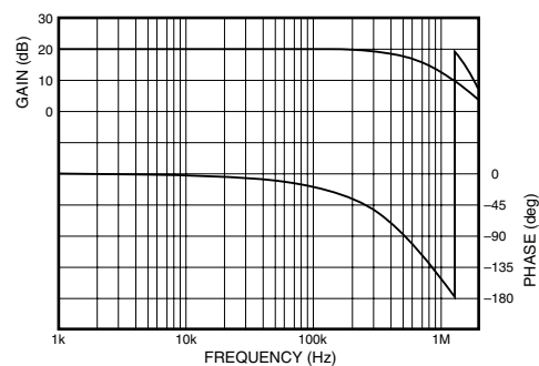
Amplitude-Phase ( \times 10 gain)
