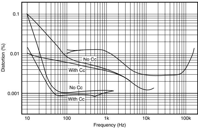
Distortion – Frequency characteristics
