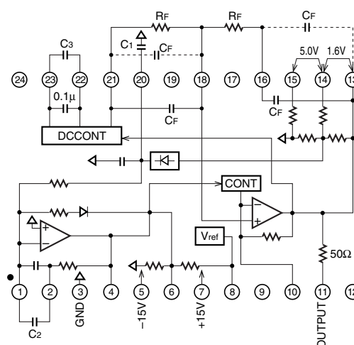
Output voltage setting
