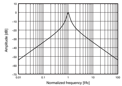
Amplitude (Band pass filter, Q = 5 )
