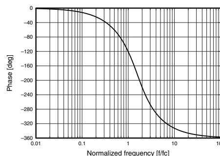
Phase characteristics
