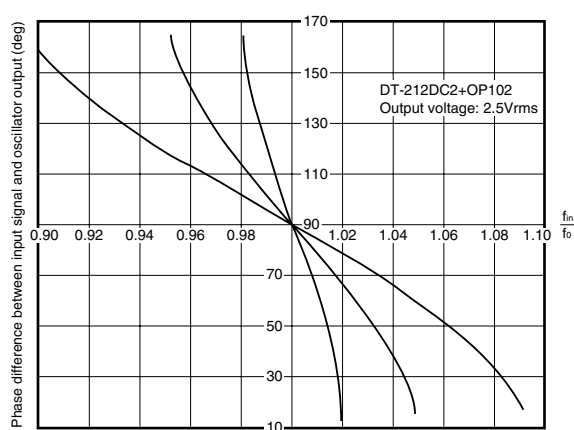
Synchronization input - Phase difference
