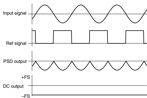
I/O waveform (Phase difference: 180^\circ )
