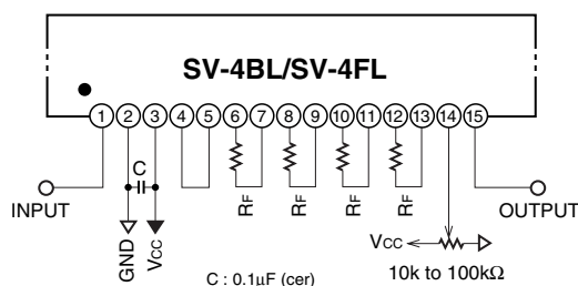
Example 1 (basic connection)
