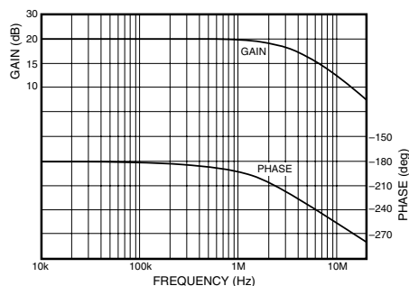
Amplitude-Phase (×20 gain)
