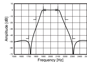
CF-4FPA 2000Hz
