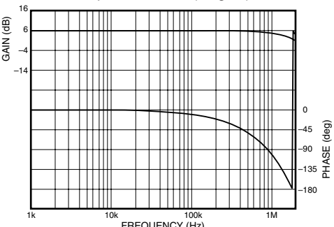
Amplitude-Phase ( \times 2 gain)
