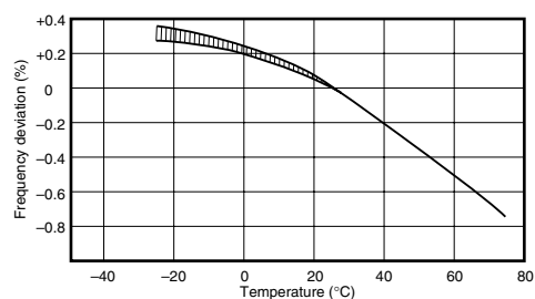
Oscillation frequency - Temperature f_o = 1\text{MHz}
