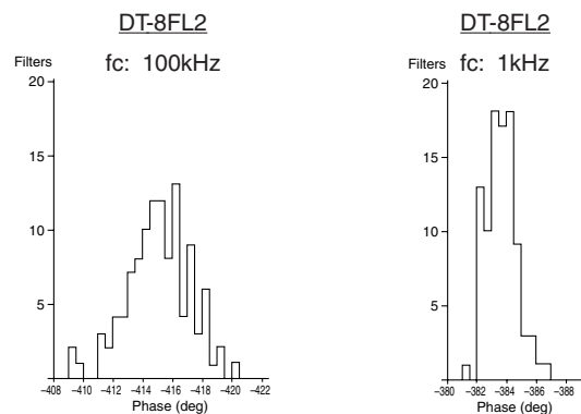
Phase matching of cut-off frequency
