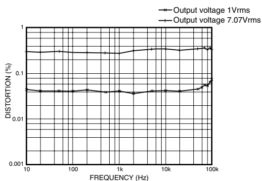
Distortion ( \times 100 gain)
