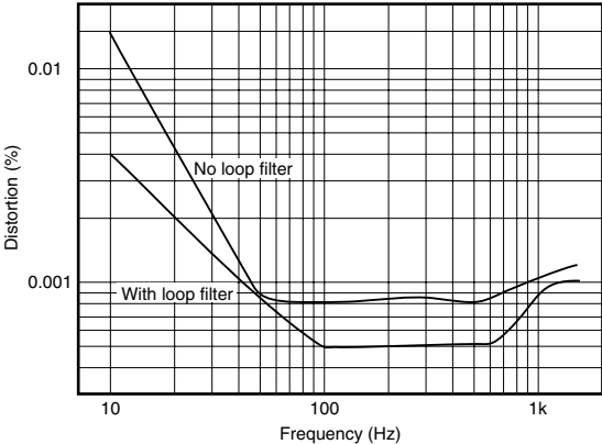
Distortion – Frequency characteristics
