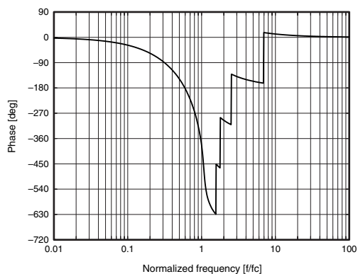
Phase
