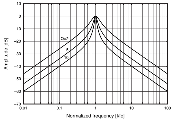
Amplitude characteristics
