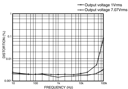
Distortion ( \times 1 gain)
