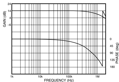
Amplitude-Phase ( \times 5 gain)
