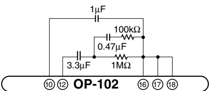
Connected with loop filter
