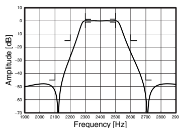
CF-4FPA 2400Hz
