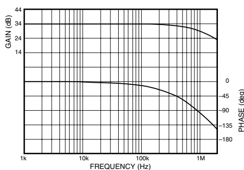
Amplitude-Phase ( \times 50 gain)
