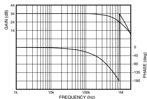
Amplitude-Phase ( \times 50 gain)
