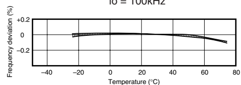
Oscillation frequency - Temperature f_o = 100\text{kHz}
