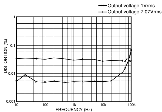
Distortion ( \times 10 gain)
