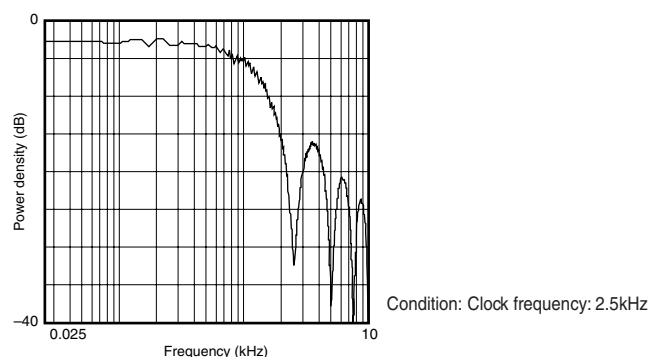
Gaussian distribution output power spectrum
