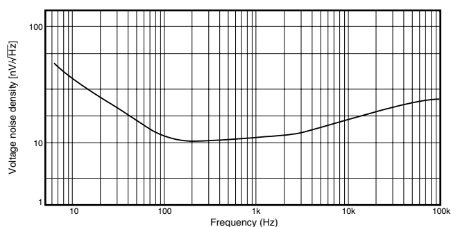
Input voltage noise density ( \times 100 gain)
