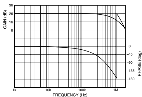
Amplitude-Phase ( \times 20 gain)
