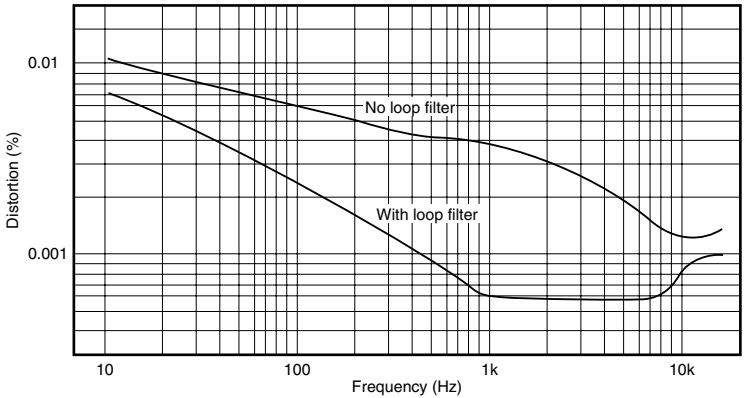
Distortion – Frequency characteristics
