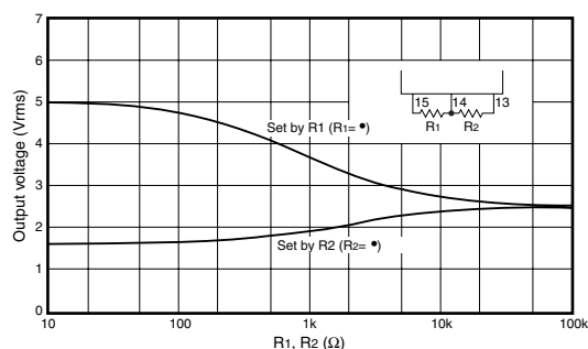
Output voltage setting
