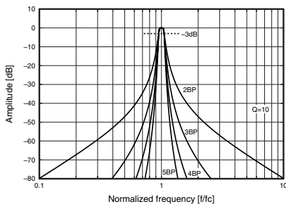
Narrow-band pass filters
