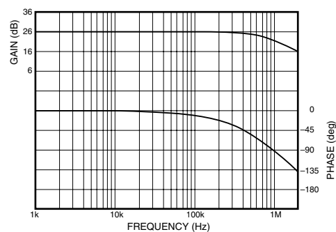
Amplitude-Phase ( \times 20 gain)
