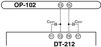
Connected with C EXT
