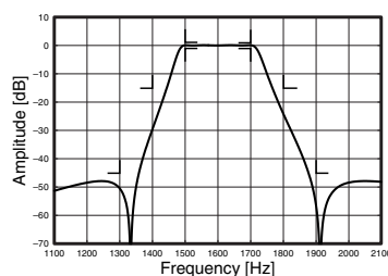
CF-4FPA 1600Hz
