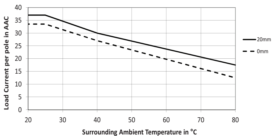
RGC3..30
