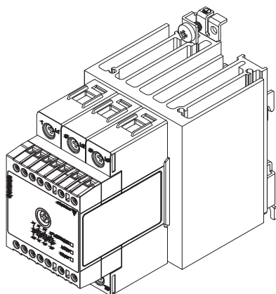
RGC2..40GGE..M RGC3..30GGE..M
