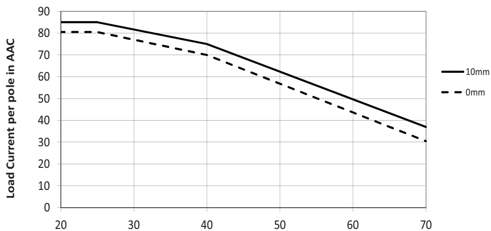
RGC2..75
