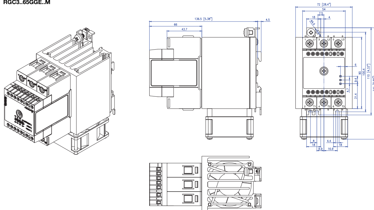
RGC2..75GGE..M RGC3..65GGE..M
