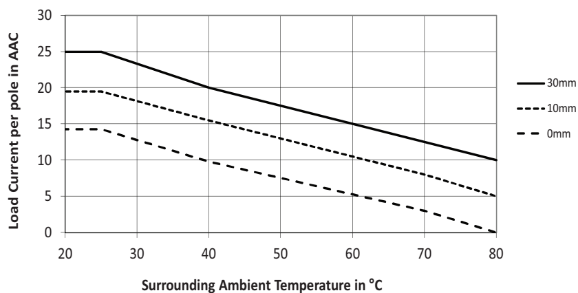
RGC3..20
