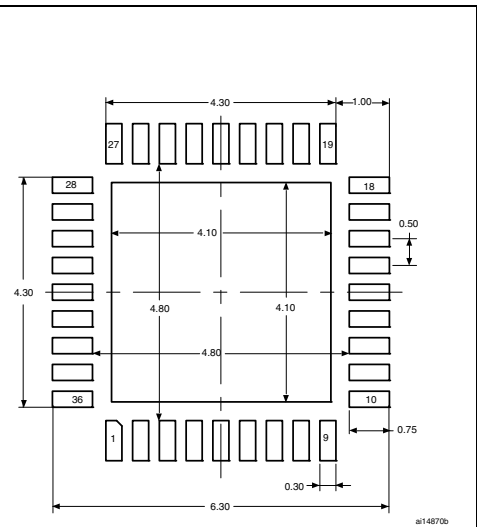
Figure 40. VFQFPN36 recommended footprint (dimensions in mm) (1)(2)
