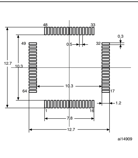
Figure 44. LQFP64 recommended footprint (1)(2)
