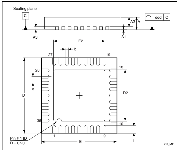
Figure 39. VFQFPN36 6 x 6 mm, 0.5 mm pitch, package outline (1)
