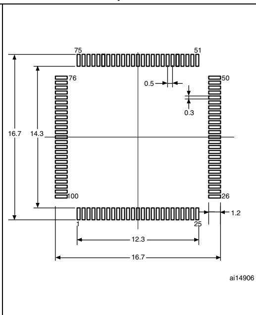
Figure 42. LQFP100 recommended footprint (1)(2)
