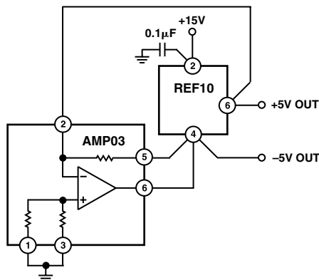
Figure 5. ±5 V Precision Voltage Reference
