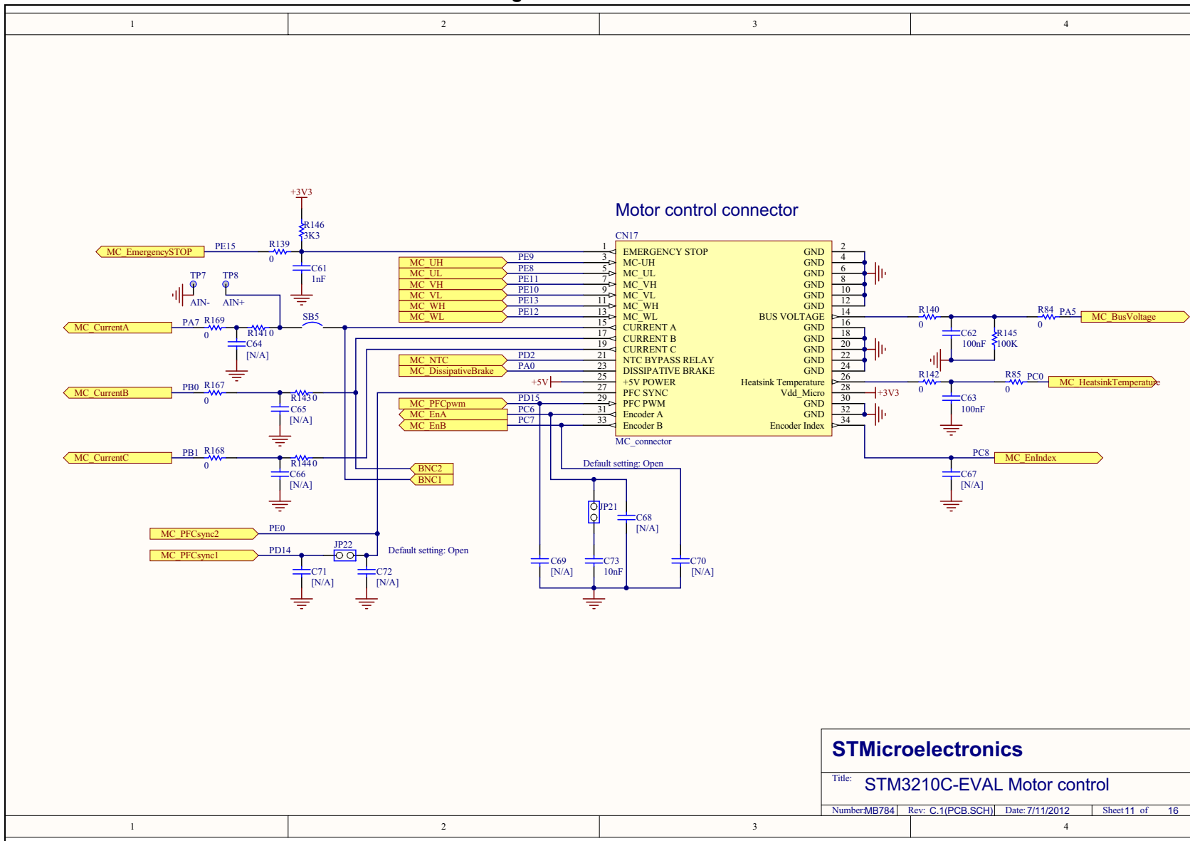
Figure 27. Motor control
