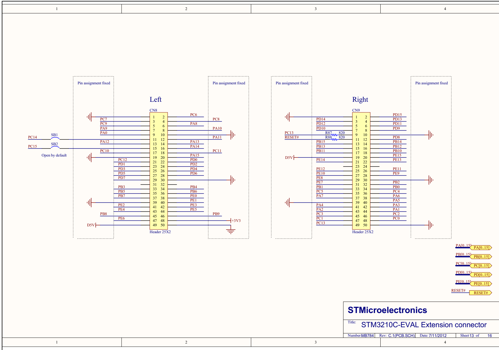
Figure 29. Extension connector
