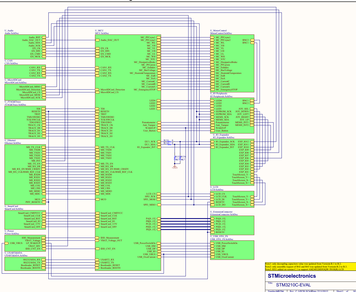
Figure 17. STM3210C
