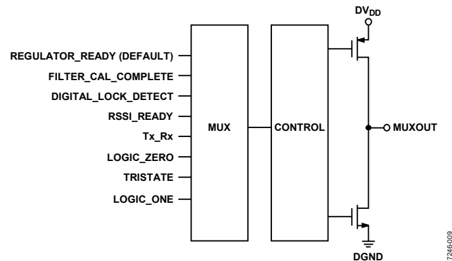
Figure 36. MUXOUT Circuit
