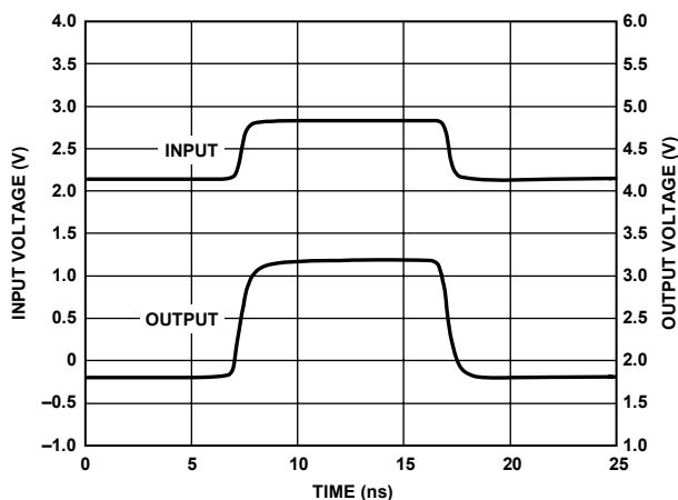
Figure 2. AD8189 Video Amplitude Pulse Response, V_{OUT} = 1.4 V p-p, R_L = 150 \Omega
