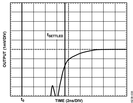
Figure 38. AD8189 Settling Time (0.1%), V_{OUT} = 2\text{ V Step} , R_L = 150\text{ }\Omega
