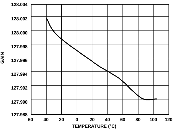
Figure 16. Gain Error (Gain = 128)
