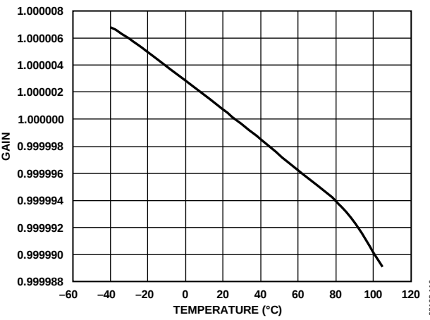
Figure 15. Gain Error (Gain = 1)
