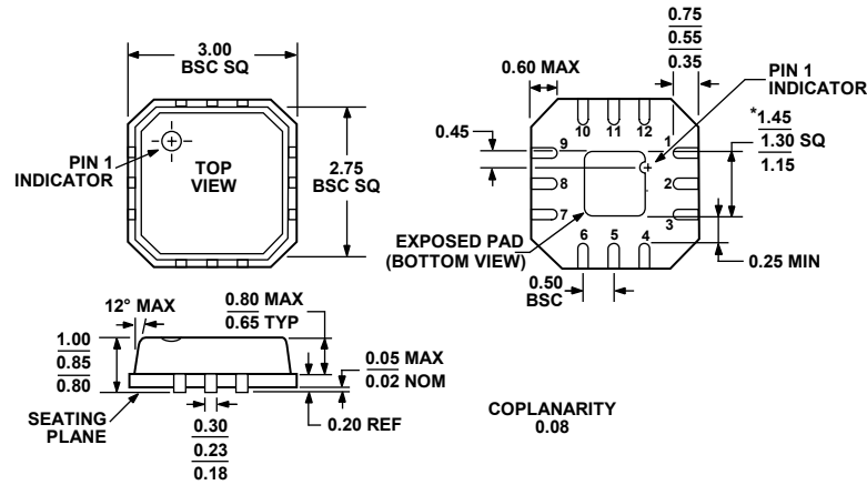
Figure 27. 12-Lead Lead Frame Chip Scale Package [LFCSP_VQ] 3 mm x 3 mm Body, Very Thin Quad (CP-12-1)
