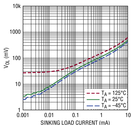
Output Saturation Voltage (V OL ) vs Load Current
