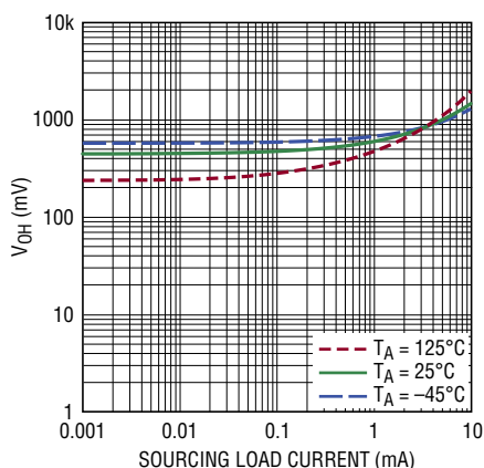
Output Saturation Voltage (V OH ) vs Load Current
