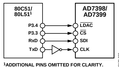
Figure 32. 80C51/80L51 to AD7398/AD7399 Interface
