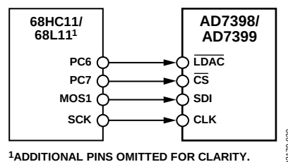
Figure 30. 68HC11/68L11 to AD7398/AD7399 Interface
