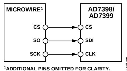
Figure 31. MICROWIRE to AD7398/AD7399 Interface
