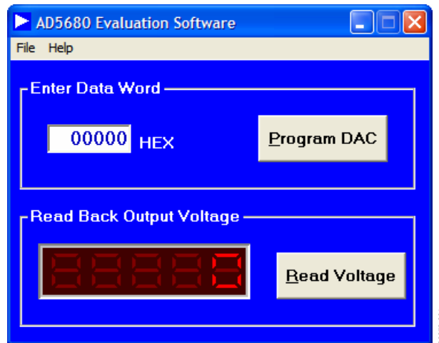
Figure 1. Main Window
