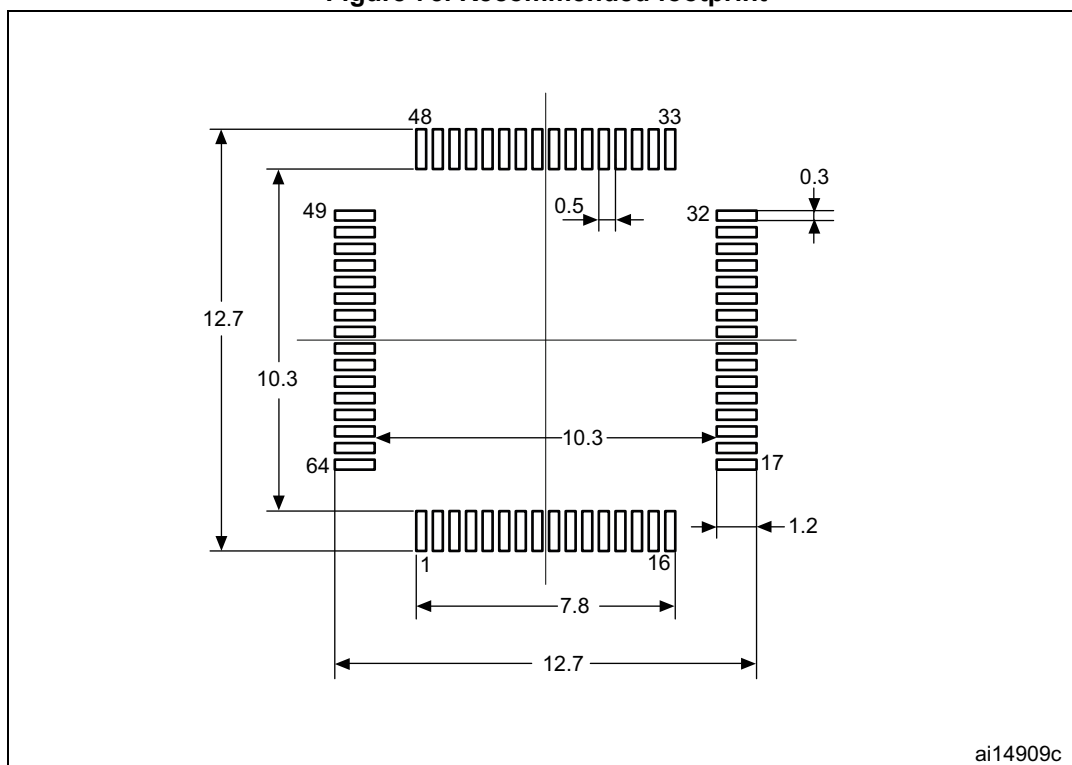
Figure 75. Recommended footprint
