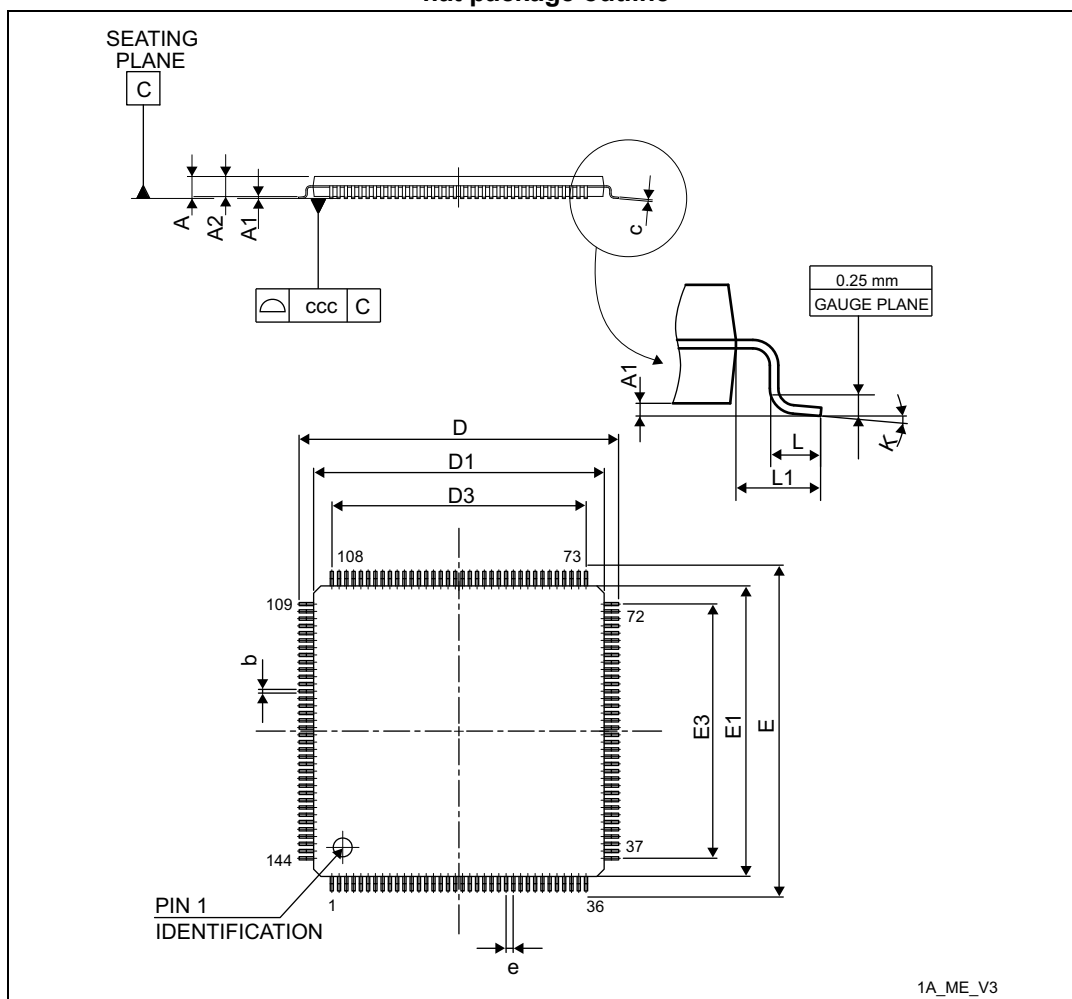
Figure 78. LQFP144, 20 x 20 mm, 144-pin low-profile quad flat package outline
