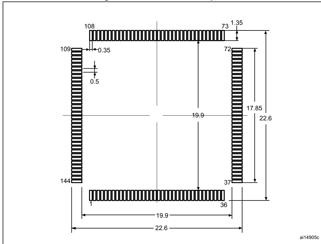
Figure 79. Recommended footprint
