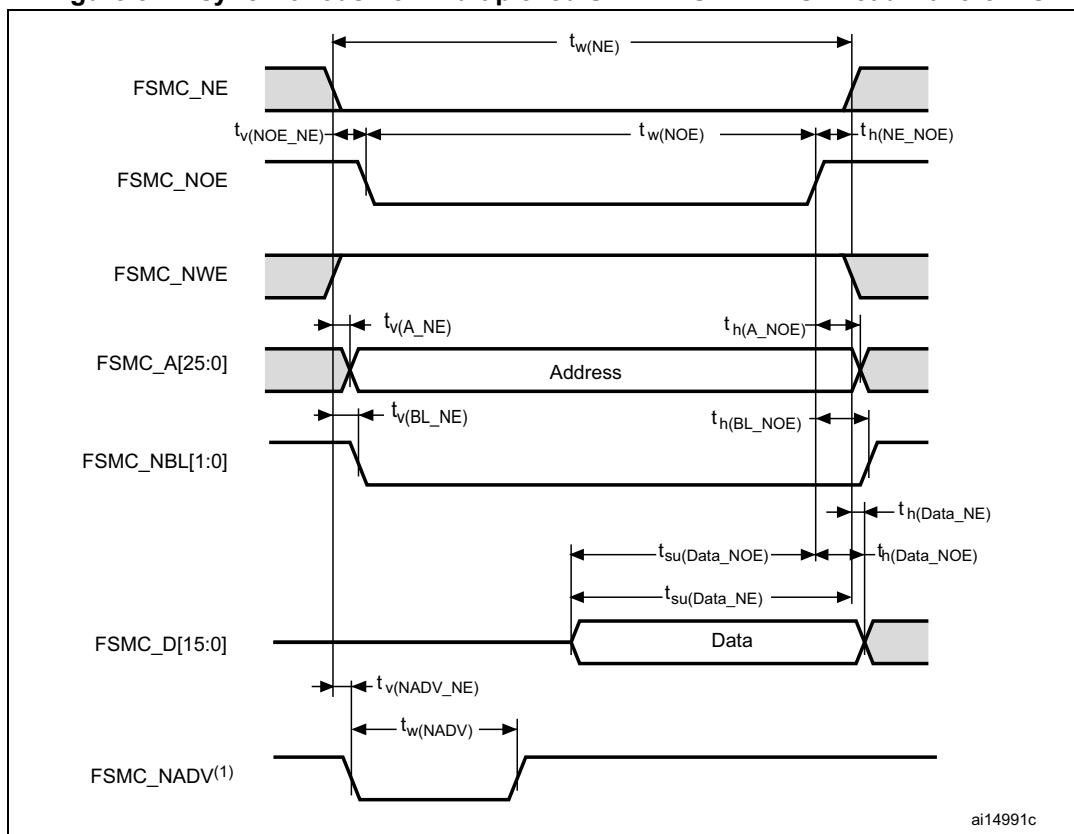
Figure 54. Asynchronous non-multiplexed SRAM/PSRAM/NOR read waveforms
