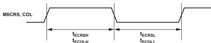
Figure 40. 10/100 Ethernet MAC Controller Timing: Asynchronous Signal
