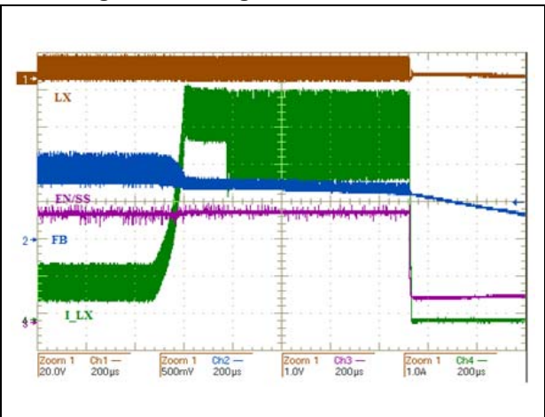
Figure 16. Long overload condition
