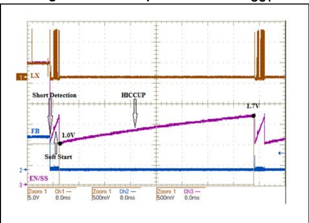
Figure 18. Start-up with shorted V_{OUT}
