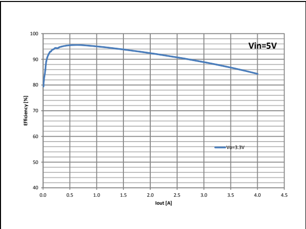
Figure 14. Efficiency vs. I_{OUT} - V_{IN} = 5\text{ V}
