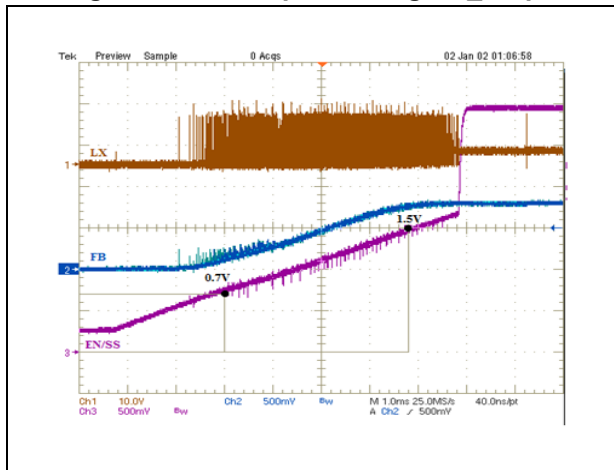
Figure 15. Start-up releasing EN_SS pin
