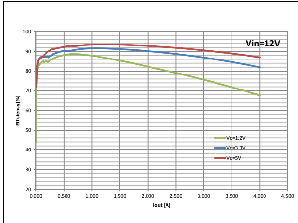
Figure 13. Efficiency vs. I_{OUT} - V_{IN} = 12\text{ V}
