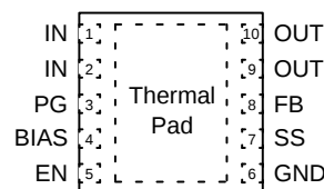
DFN10-3x3-0.5P
