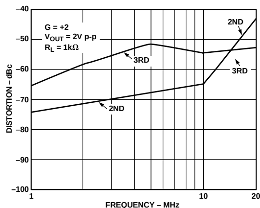
Figure 13. Distortion vs. Frequency V_S = +5\text{ V}
