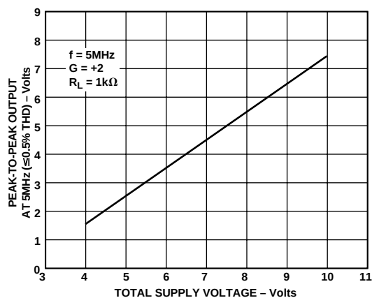
Figure 15. Output Swing vs. Supply
