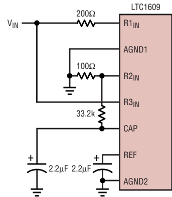
Figure 3a. Offset/Gain Circuits for Unipolar Input Ranges
