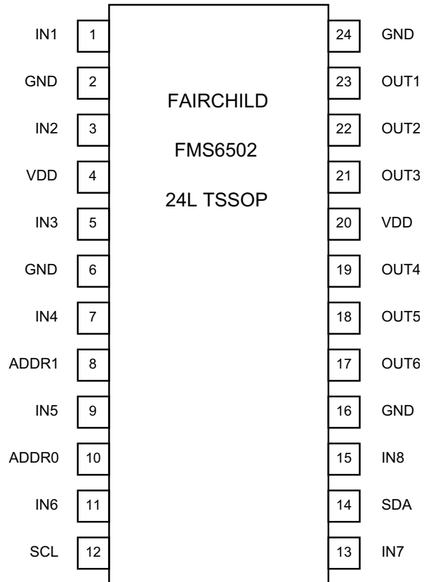
Figure 2. Pin Configuration
