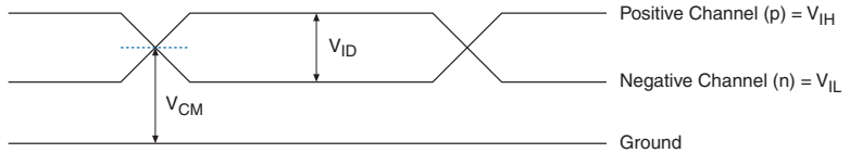
Figure 5–1. Receiver Input Waveforms for Differential I/O Standards
