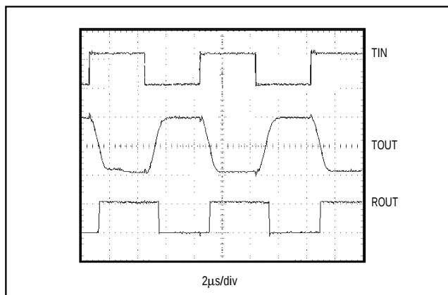
Figure 4. Loopback Test Results at 250kbps
