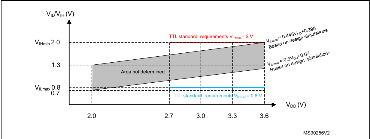
Figure 20. TC and TTa I/O input characteristics - TTL port
