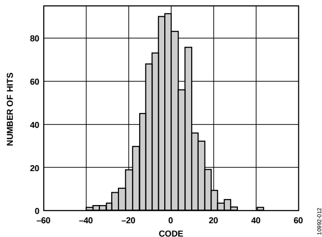
Figure 12. Channel Offset Distribution (Gain = 17 dB)
