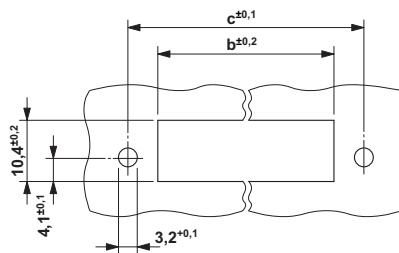
Dimensioned drawing
