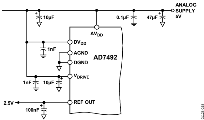
Figure 28. Typical Decoupling Circuit
