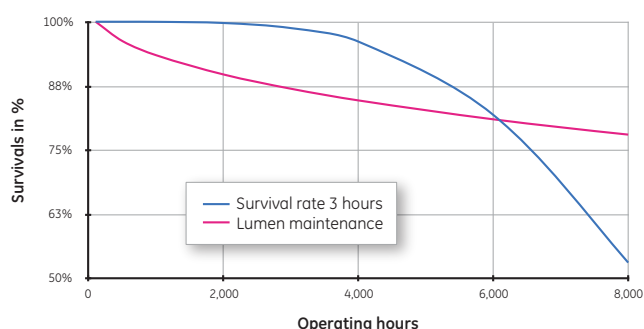
Life expectancy and lumen maintenance T2 Spiral 8,000 hours
