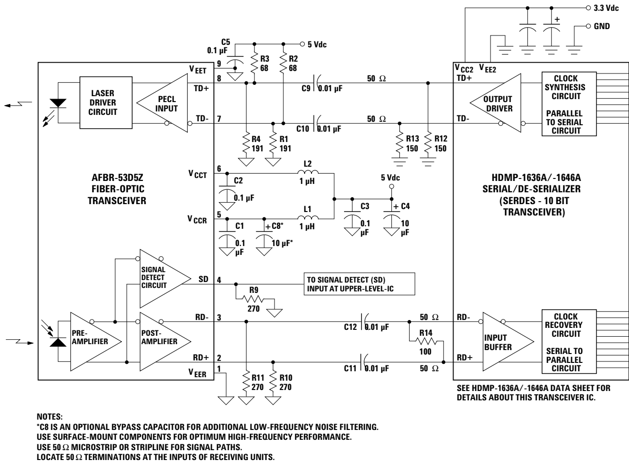
Figure 3. Recommended Gigabit/sec Ethernet AFBR-53D5Z Fiber-Optic Transceiver and HDMP-1636A/1646A SERDES Integrated Circuit Transceiver Interface and Power Supply Filter Circuits.
