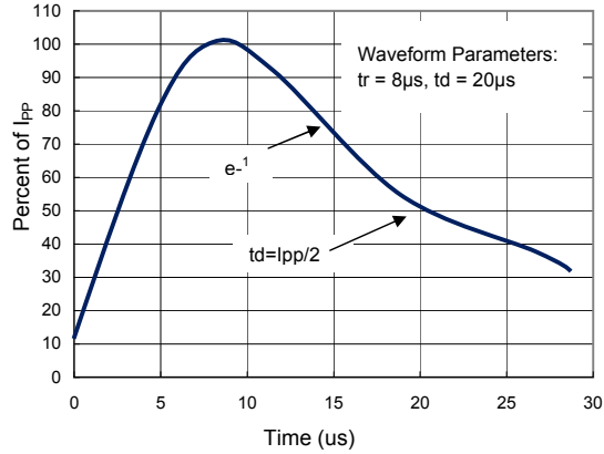
FIG 2 Pulse Waveform
