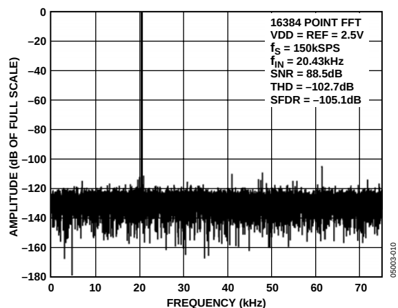
Figure 10. FFT Plot
