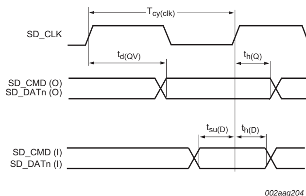
Fig 36. SD/MMC timing
