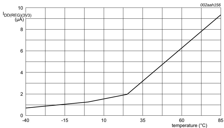
Fig 16. Typical supply current versus temperature in Deep power-down mode
