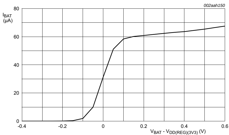
Fig 17. Typical battery supply current in Active mode
