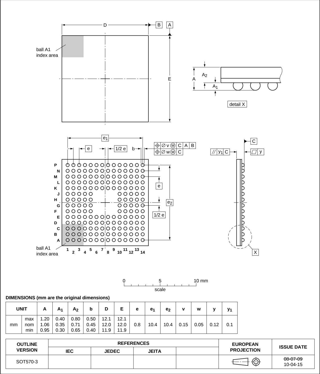
Fig 49. Package outline of the TFBGA180 package
