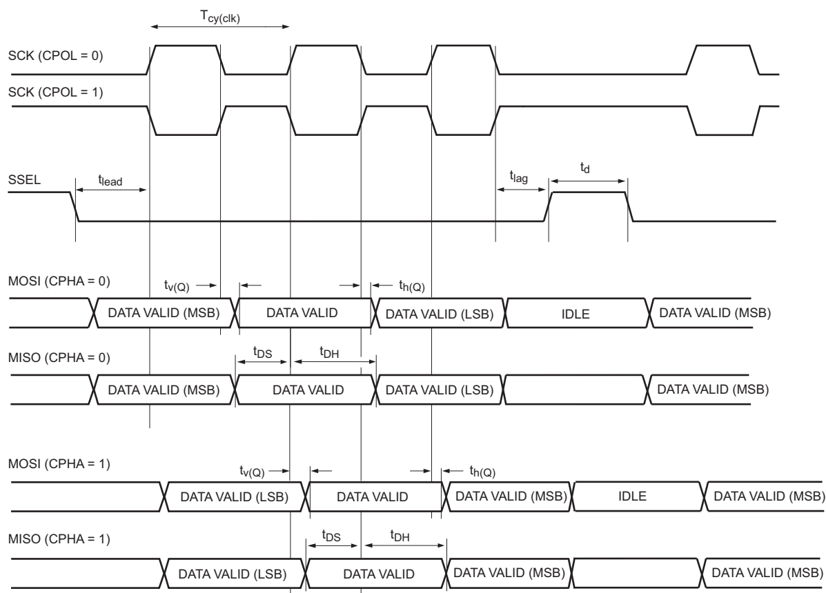
Fig 29. SSP master timing in SPI mode
