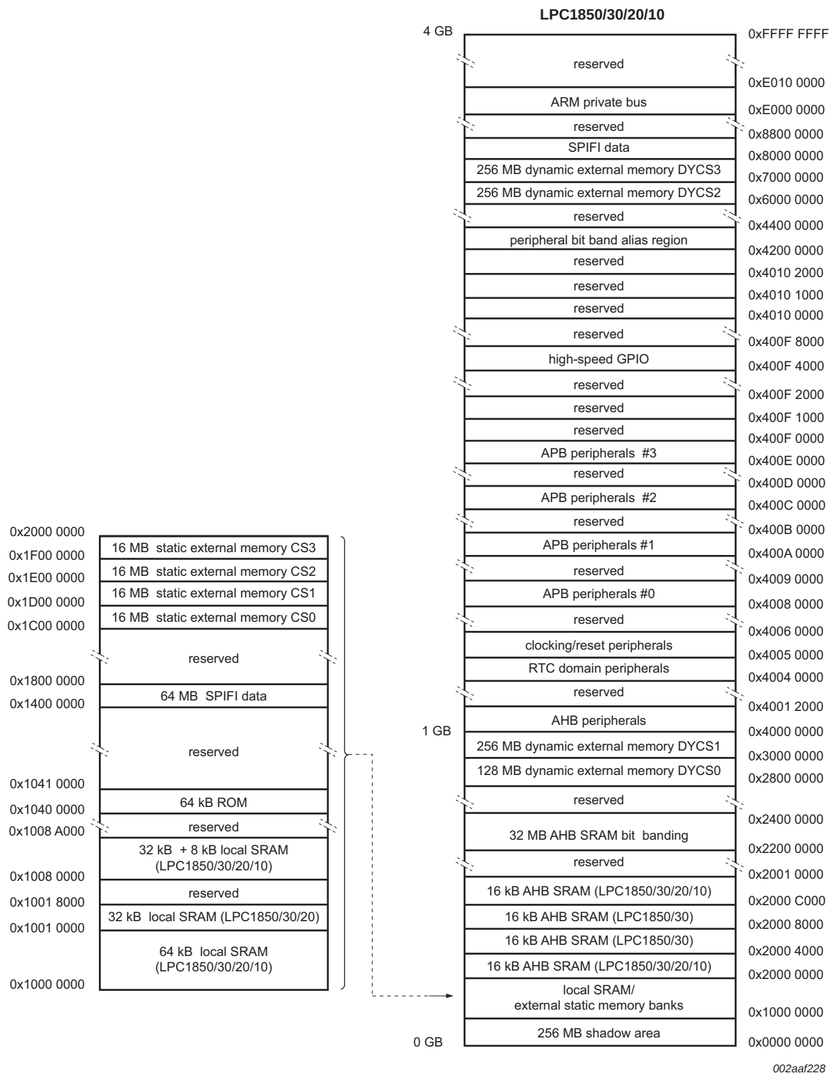
Fig 7. LPC1850/30/20/10 Memory mapping (overview)
