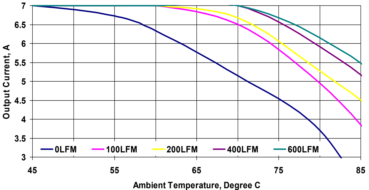
Figure 17. Thermal Derating Curves. Vin=14V, Vout=5.0V
