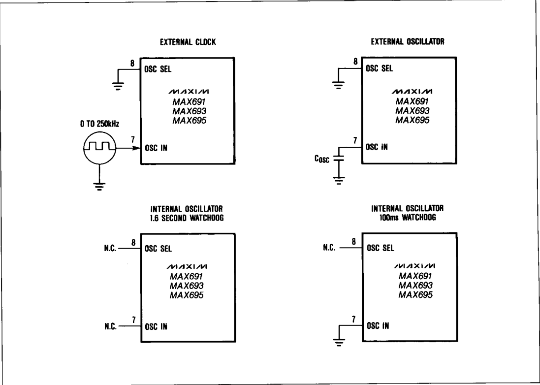
Figure 8. Oscillator Circuits
