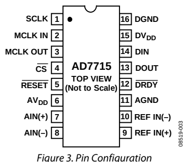
Figure 3. Pin Configuration
