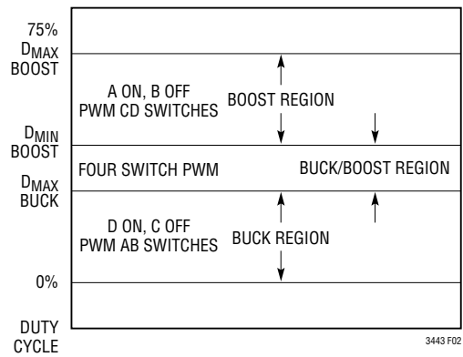
Figure 2. Switch Control vs Internal Control Voltage, V_{CI}
