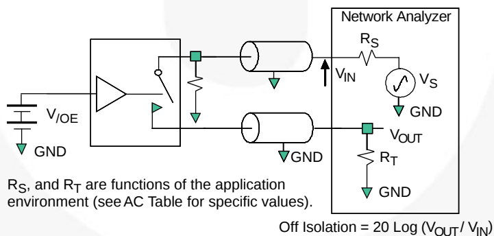
Figure 15. Channel Off Isolation
