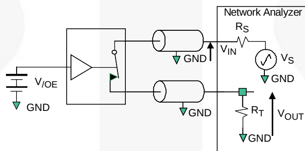
Figure 14. Bandwidth
