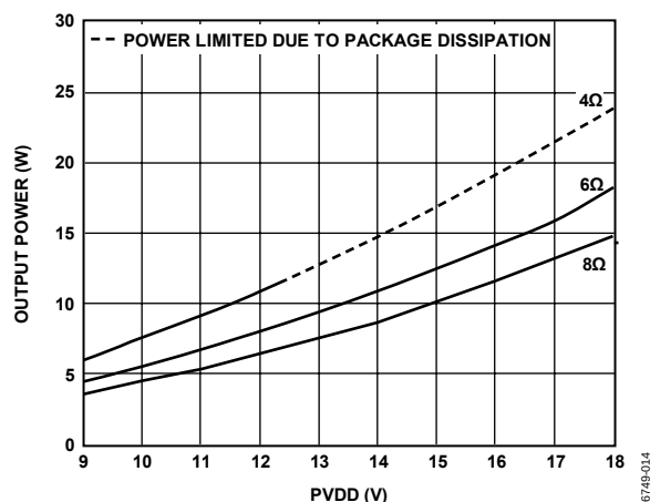
Figure 14. Output Power vs. PVDD @ 0.1% THD + N
