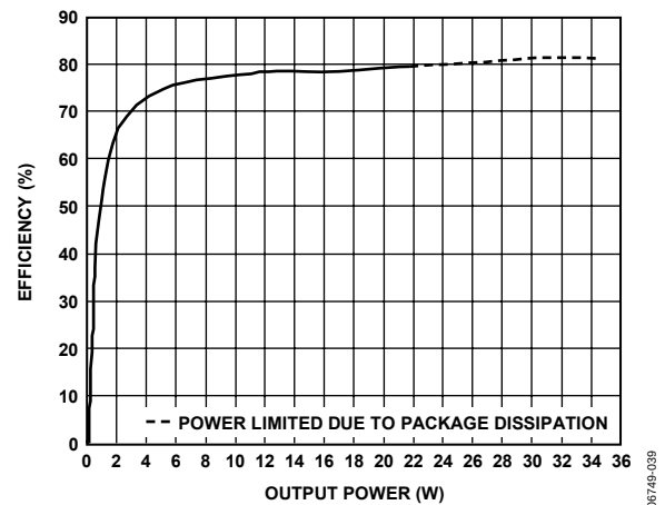
Figure 39. Efficiency vs. Output Power, Mono Mode, 15 V, 3 Ω
