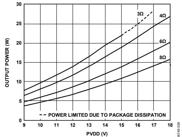
Figure 38. Output Power vs. PVDD, Mono Mode, 60 dB THD + N
