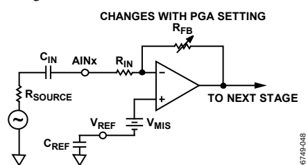
Figure 48. Input Equivalent Circuit
