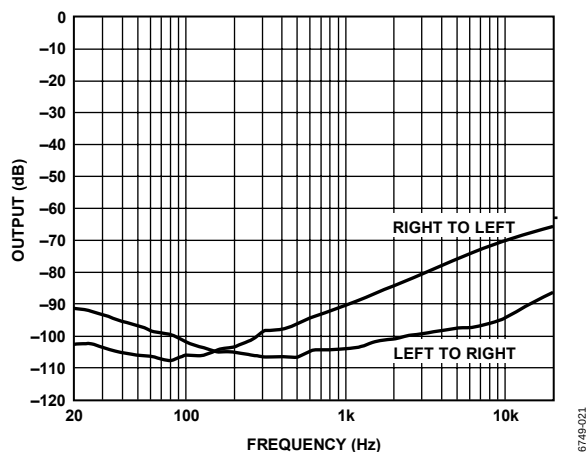
Figure 21. Crosstalk @ 1 W, 6 \Omega , PVDD = 15 V, PGA = 0 dB
