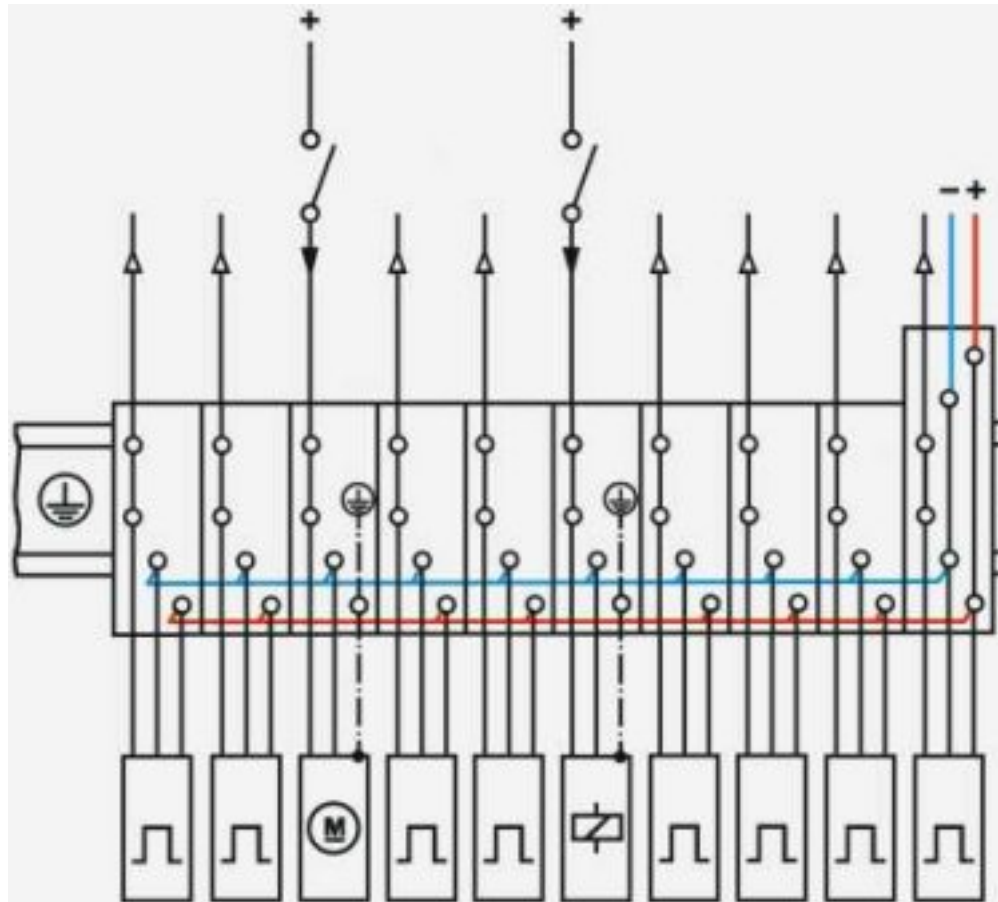
Circuit diagram
