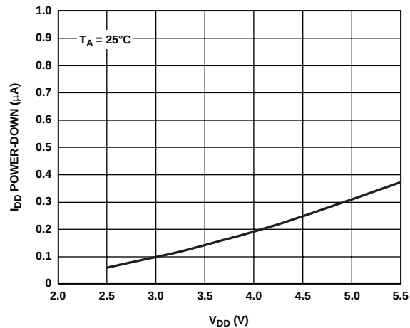
Figure 27. Power-Down Current vs. Supply Voltage
