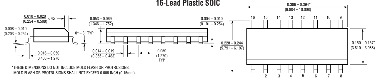
S Package 16-Lead Plastic SOIC
