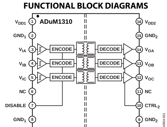
Figure 1. ADuM1310
