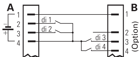
Supply voltage for energization of digital input (e.g. di1...di4)
