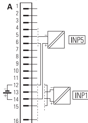
Connection of a 2-wire transmitter on example of INP1 or INP5
