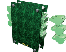
Plug-in terminal 3 Level 2 PCB + BUS 45 mm
