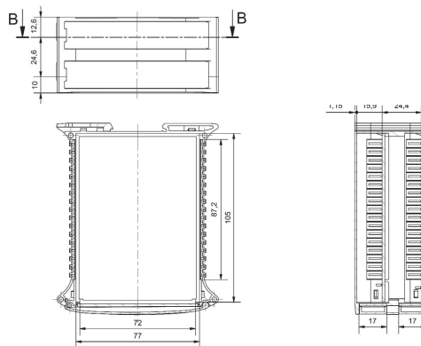
Altezza max comp. 20 mm / Max components height 20 mm Dimensione in mm (tolleranze ± 0,2mm) / Dimensions in mm (tolerances ± 0,2mm)
