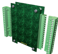
Standard Plug-in terminal 2 PCB + BUS 35 mm
