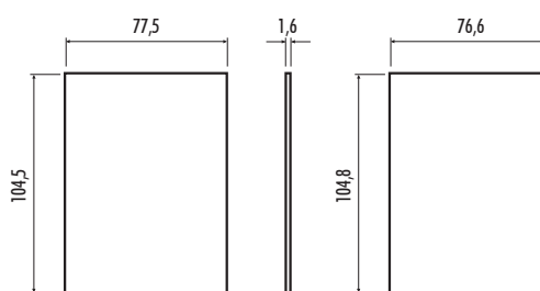
Circuito stampato RAILBOX RAILBOX Printed Circuit Board
