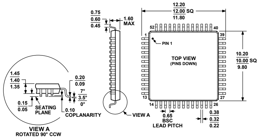
Figure 49. 52-Lead Low Profile Quad Flat Package [LQFP] (ST-52) Dimensions shown in millimeters
