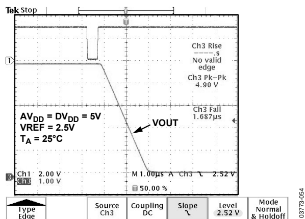
Figure 25. AD539x Slew Rate Boost On
