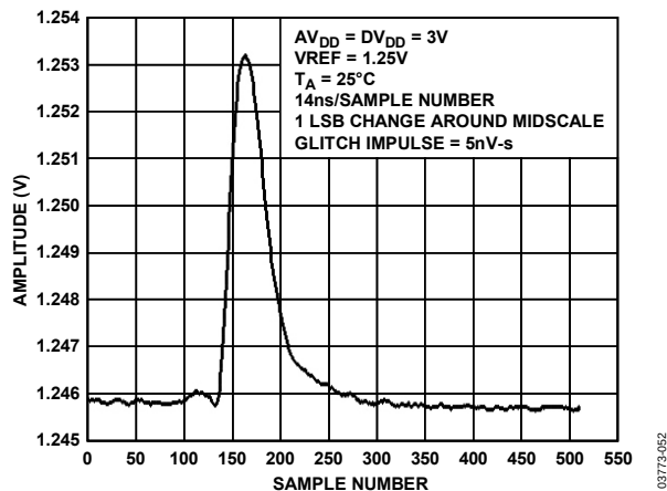
Figure 23. AD539x-3 Glitch Impulse
