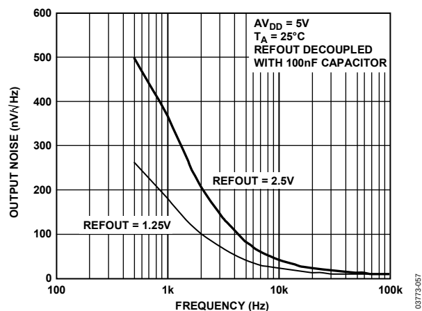
Figure 28. AD539x REFOUT Noise Spectral Density
