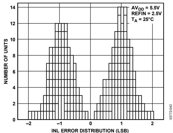
Figure 12. AD5390-3/AD5392-3 INL Plot
