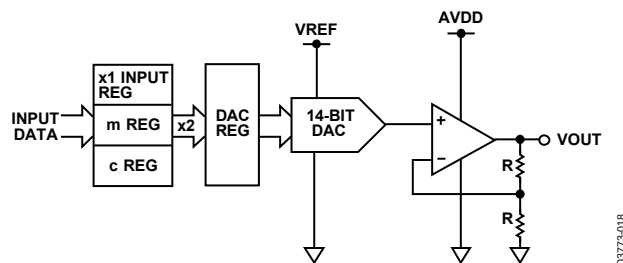
Figure 31. Single-Channel Architecture
