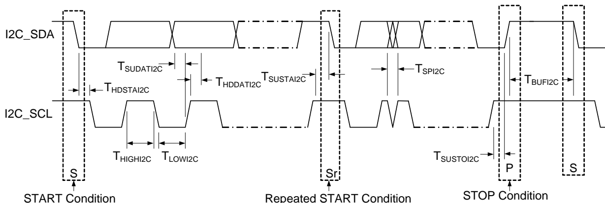
Figure 6-8. Definition for Timing for Fast-/Standard-Mode on the I 2 C Bus
