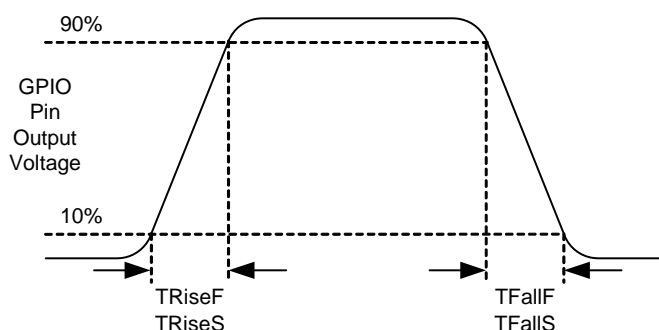
Figure 1. GPIO Timing Diagram
