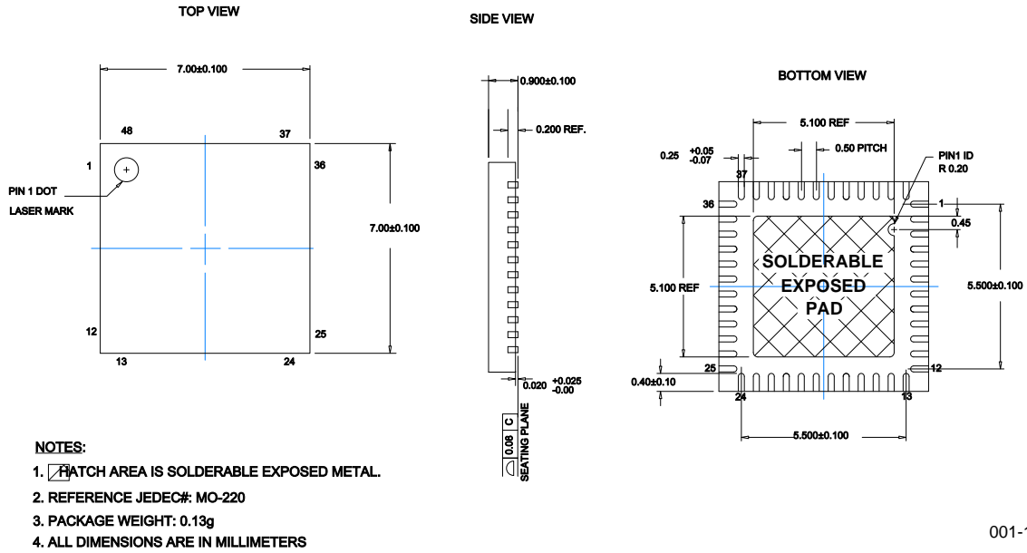
Figure 7-4. 48-Pin (7 x 7 x 1.0 mm) QFN (Sawn)
