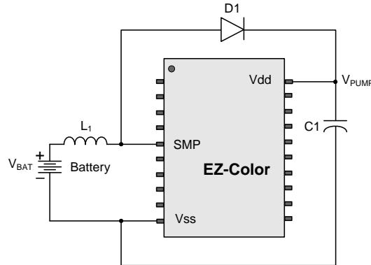
Figure 6-2. Basic Switch Mode Pump Circuit
