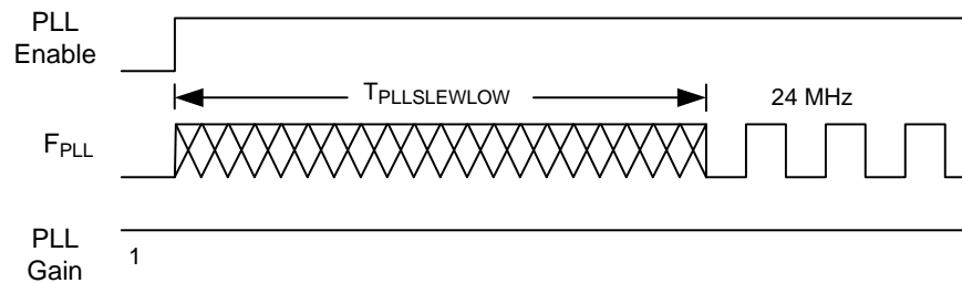
Figure 6-4. PLL Lock for Low Gain Setting Timing Diagram
