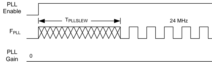
Figure 6-3. PLL Lock Timing Diagram
