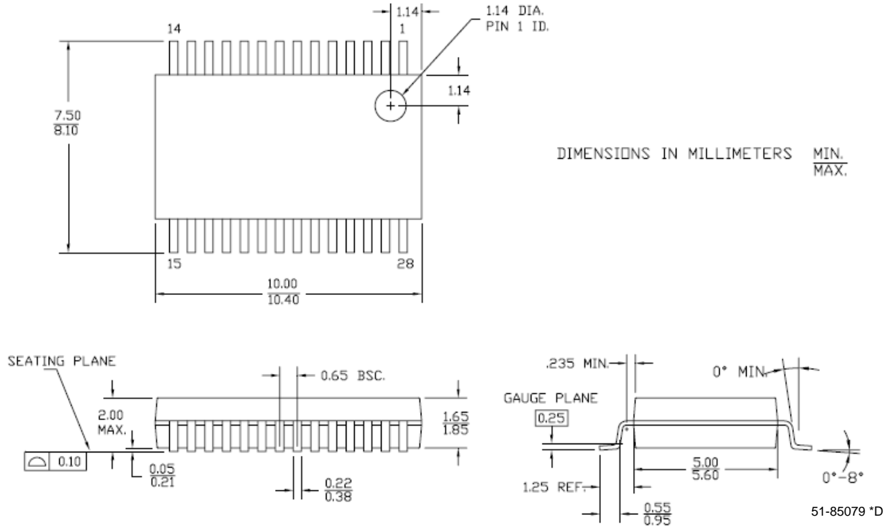
Figure 7-1. 28-Pin (210-Mil) SSOP
