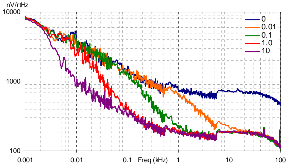
Figure 6-6. Typical AGND Noise with P2[4] Bypass
