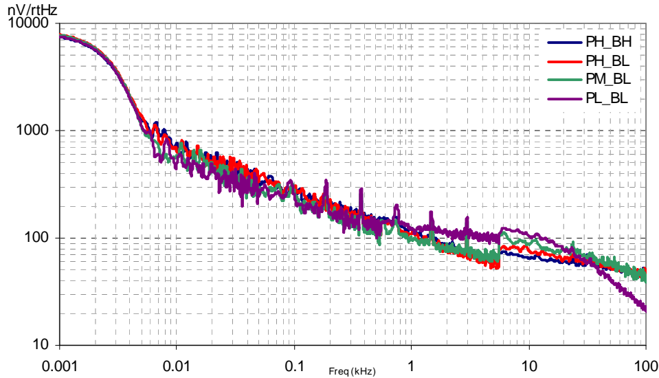
Figure 6-7. Typical Opamp Noise
