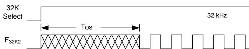
Figure 6-5. External Crystal Oscillator Startup Timing Diagram
