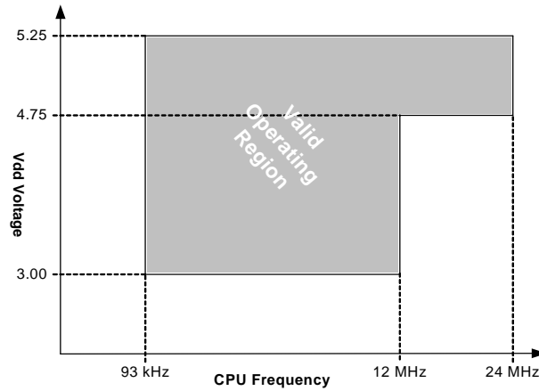
Figure 6-1. Voltage vs. CPU Frequency
